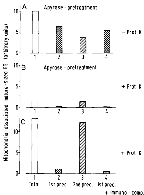
Fig.1. F 1 \beta accumulated in translocation contact sites is accessible to antibodies added to isolated mitochondria. In experiment A, isolated Neurospora mitochondria and rabbit reticulocyte lysates containing radiolabelled mitochondrial precursor proteins were pre-treated with apyrase (0.7 U/ml) as described [22]. The mitochondria were added to the reticulocyte lysate in the presence of 8 mM ascorbate, 0.2 mM N,N,N',N'-tetramethylphenylenediamine (TMPD), and 6 mM ADP as in [12,13]. After 20 min at 25°C, mitochondria were re-isolated. Mitochondria from one aliquot were lysed in 1% (w/v) Triton X-100, and F 1 \beta was immunoprecipitated (sample 1). With a second aliquot, the re-isolated mitochondria were incubated with antibodies against F 1 \beta (30 min at 0°C). Mitochondria were re-isolated, lysed in 1% Triton X-100 and antibody-F 1 \beta complexes were harvested, after addition of protein A-Sepharose, by centrifugation. Radiolabelled m-F 1 \beta was determined as described in section 2 (sample 2). The supernatant of this reaction ('1st prec.') again received antibodies against F 1 \beta and a second immunoprecipitation was performed ('2nd prec.') (sample 3). Reaction 4 was performed as described for sample 2 except that the mitochondria were lysed in the presence of an excess of unlabelled mitochondria ('immunocomp.'). Experiment B was performed as described for A except that the mitochondria were treated with proteinase K (20 \mu g/ml; Prot K) after the import incubation as described [12]. Experiment C was performed as described for B except that the pre-treatment with apyrase and the addition of ADP were omitted, and that the import incubation was performed for 40 min at 25°C.
